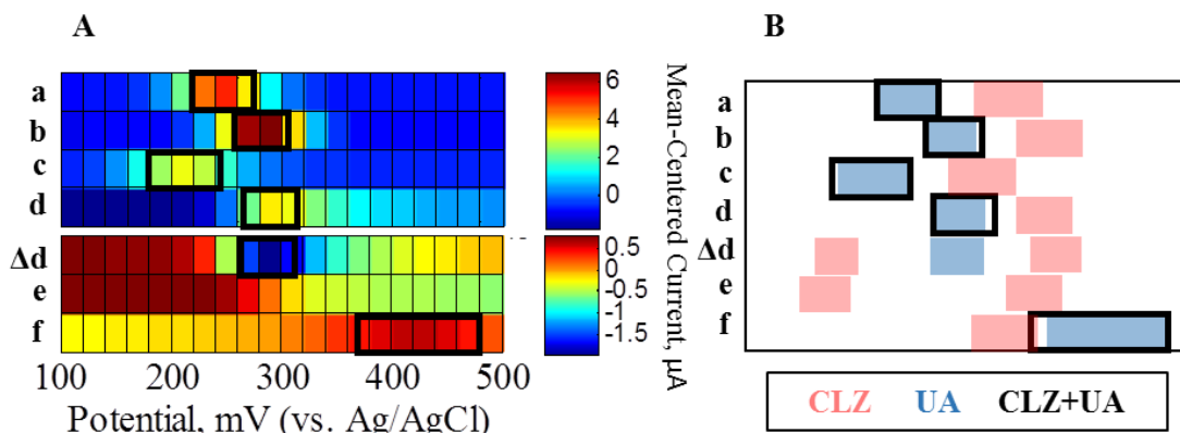
Figure 21. (A) Heat map representation of electrochemical responses of the CRS (elements a-f) for 410 µM UA tested individually. Black outlines represent the location of peaks. (B) Simplified heat map showing the electrochemical peak locations of 410 µM UA tested individually in mixture with 5.6 µM CLZ, as well as control 5.6 µM CLZ tested individually for comparison, in PBS buffer. Each response represents the average absolute value of triplicate measurements. Each heat map contains an individual color scale.
