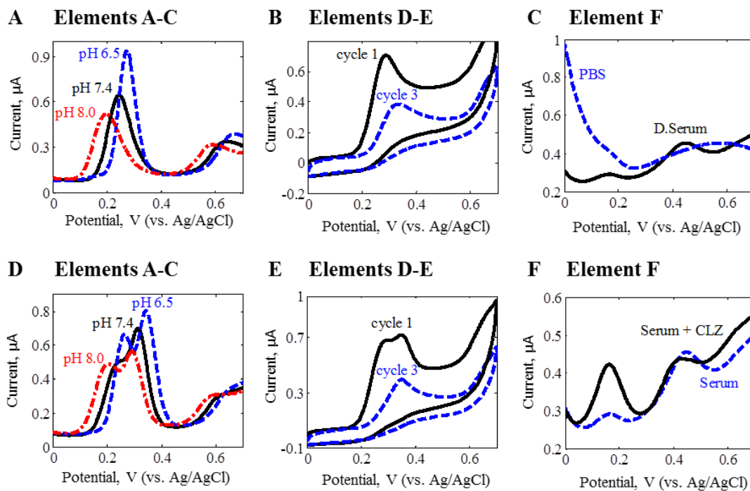
Figure 26. The CRS responses of deproteinized serum are shown across the various sensing element. (A) Serum DPV signals at pH 6.5, 7.4 and 8.0 (elements A – C) using a GCE, (B) serum CV signal at pH 7.4 using GCE for cycles 1 – 3 (elements D – E), and (C) serum DPV signal with the Pt electrode (element F) is compared to background reactions of PBS at pH 7.4. (D) CLZ-spiked serum DPV signals at pH 6.5, 7.4 and 8.0 (elements A – C) using a GCE, (E) CLZ-spiked serum CV signal at pH 7.4 using GCE for cycles 1 – 3 (elements D – E), and (E) CLZ-spiked serum DPV signal with the Pt electrode (element F) is compared to background reactions of serum at pH 7.4. The A – F annotations refer to the various elements in the CRS (Table 5), and the proteins were removed from serum samples. Each curve represents the average of duplicate measurements.
