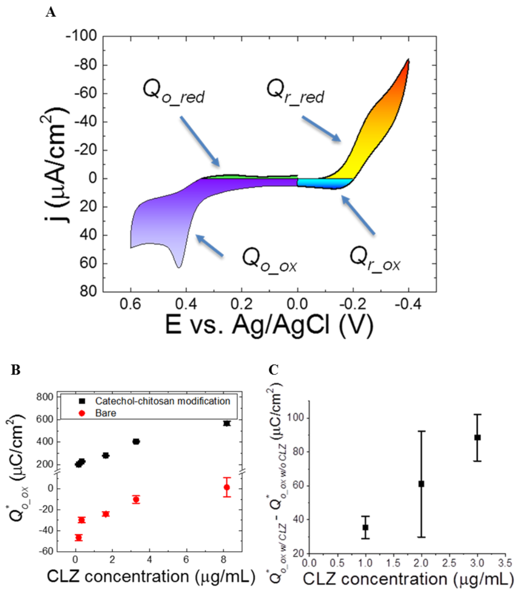
Figure 7. Calibration of CLZ at ccRCS Electrodes. (a) Cyclic voltammogram response divided into 4 sections, Q_{r\_red} (red-yellow) for cathodic charge at E < 0 V (Ru reduction), Q_{r\_ox} (blue) for anodic charge at E < 0 V, Q_{o\_ox} (purple) for anodic charge at E > 0 V (CLZ oxidation), and Q_{o\_red} (green) for cathodic charge at E > 0 V. The Q_{o\_ox} section was correlated to CLZ concentration in (b) buffer solutions using bare and catechol-chitosan modified electrodes, as well as in (c) serum solutions using catechol-chitosan modified electrodes. Measurements were carried out in duplicates using an on-chip setup [74].
