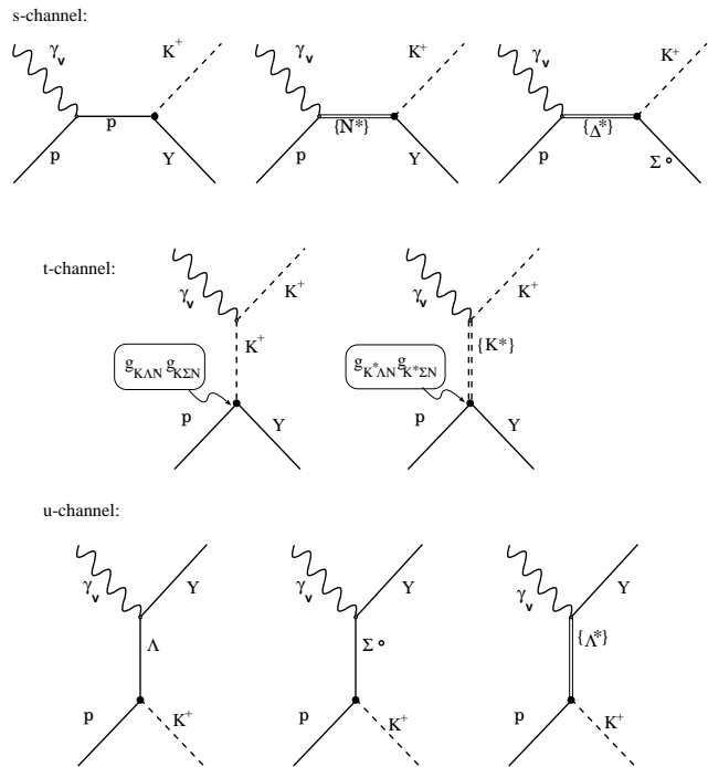
FIG. 1: Examples of Feynman diagrams for kaon electroproduction considered in the isobaric models. The couplings in the t -channel ( g_{K\Lambda N} , etc...) are shown explicitly. Note that the s -channel processes involving \Delta^* resonances are forbidden by isospin conservation for \Lambda production.
