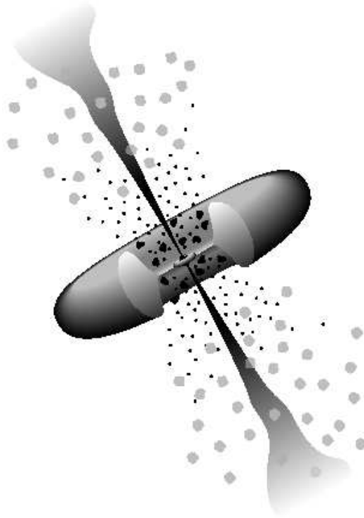
Figure 2.1: Cartoon model of an AGN. A central super-massive black hole is surrounded by an accretion disk. The region may be surrounded by clouds which exhibit broad-line emission closer to the center and narrow-line emission further away. A dusty torus may also surround the center, obscuring broad-line emission from some lines of sight. Radio, X-ray, and gamma-ray emission may be viewed from extended particle jets depending on the observation angle. Figure from Urry & Padovani (1995).
