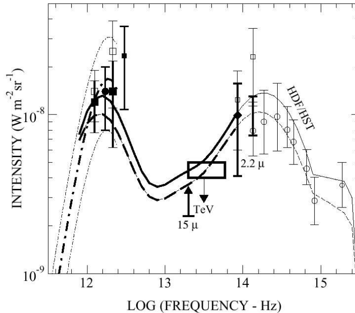
Figure 2.4: Measurements and models of the extragalactic background. The solid and dashed curves correspond to luminosity evolution models from Malkan & Stecker (2001). The frequency range that can be constrained with TeV observations of AGN is marked. Figure taken from Konopelko et al. (2003).
