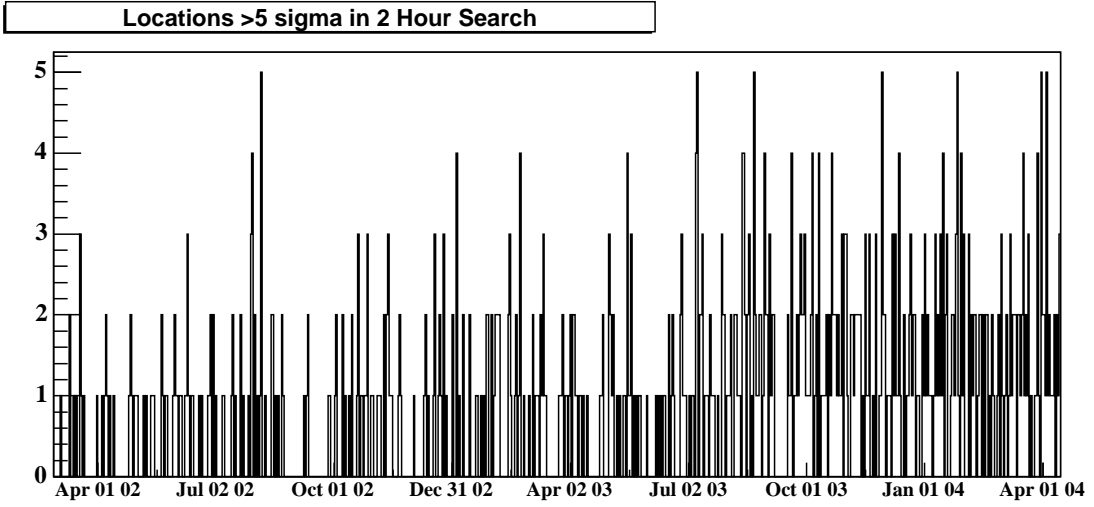
Figure 7.8: Time distribution of two-hour alerts with Z_{LM} > 5 from 27 February 2002 to 16 April 2004.
