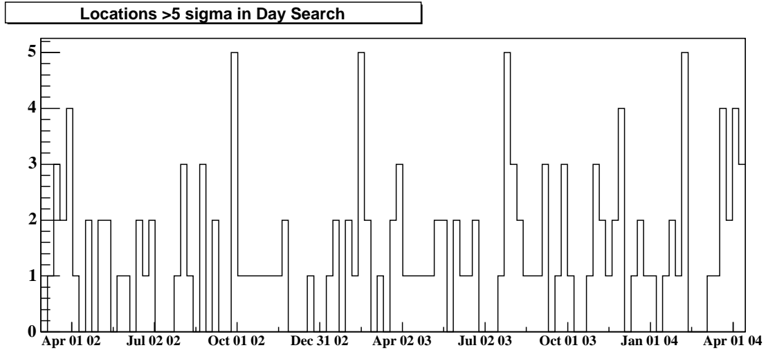
Figure 7.9: Time distribution of one-day alerts with Z_{LM} > 4.8 from 27 February 2002 to 16 April 2004.
