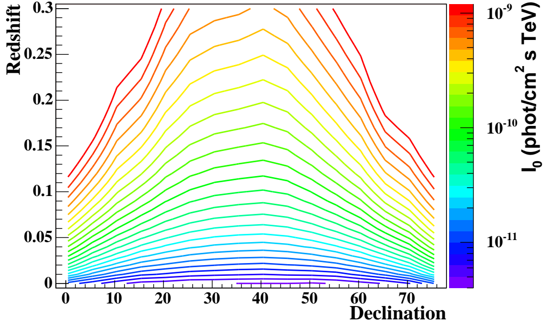
Figure 8.2: Differential flux amplitude, I_0 in dN/dE = I_0(E/\text{TeV})^{-\alpha}e^{-\tau(E,z)} with \alpha = 2.0 , necessary for a 3\sigma observation of a source at the given declination and redshift in 906 days. The redshift attenuation is obtained using IR1a.
