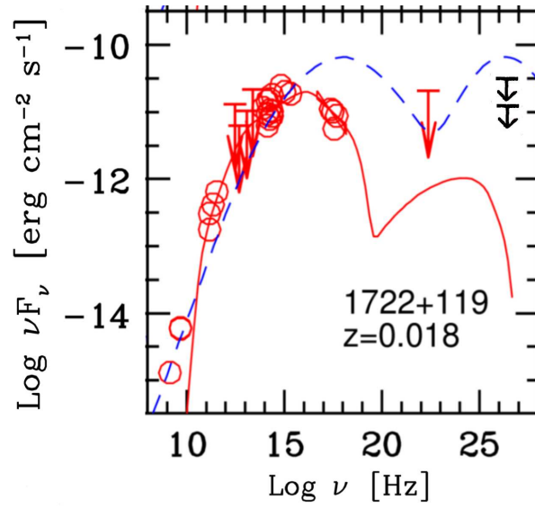
Figure 8.5: SED data and predicted SSC (solid) and Fossati (dashed) fits for RGB 1725+118 from Costamante & Ghisellini (2002). The Milagro flux upper limits for an unabsorbed (lower) and absorbed (higher) spectrum are in black.
