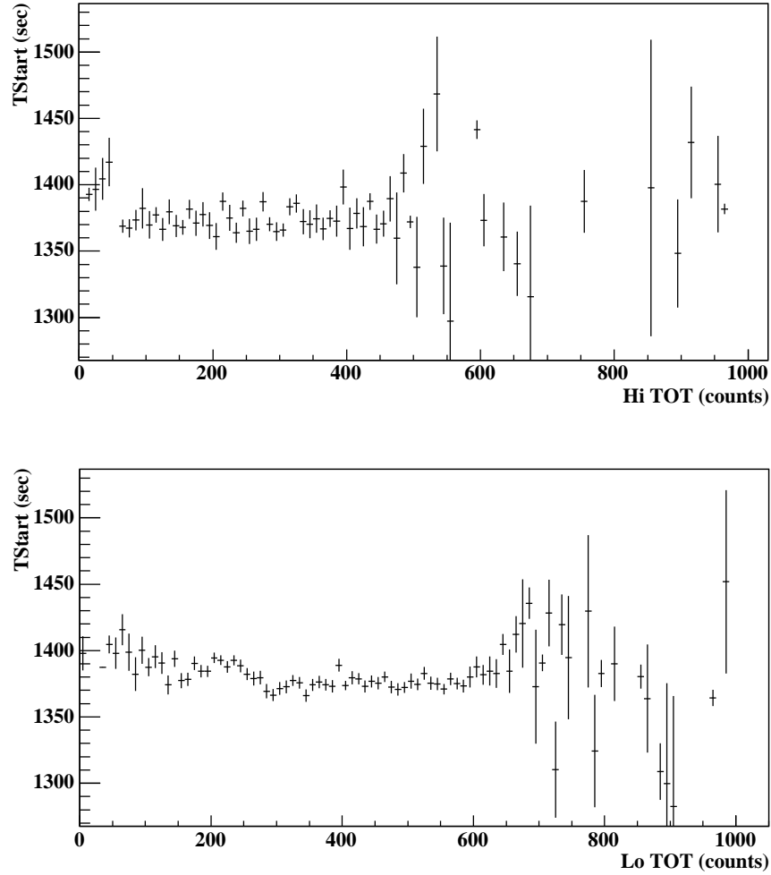
Figure 4.8: Calibrated TStart as a function of Hi and Lo TOT for an AS PMT. The calibrated time has the slewing correction and, thus, the pulse amplitude dependence removed. The times for both the high and low thresholds also appear at the same level in TStart.
