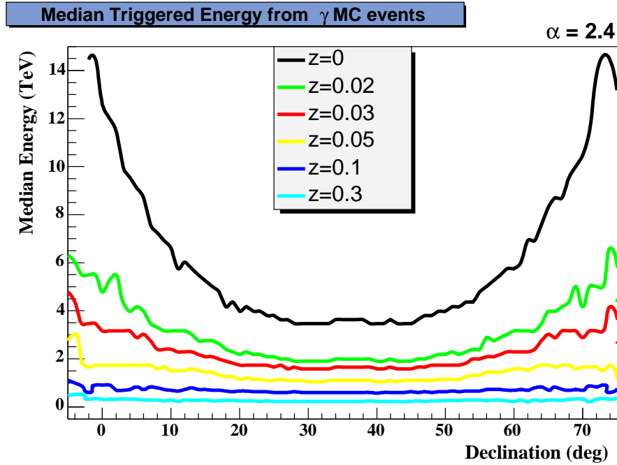
Figure 6.8: Median energy for dN/dE \propto E^{-2.4}e^{-\tau(E,z)} using IR1a. The energy flattens in declination with redshift, but the source sensitivity (fig 6.9) shows that as redshift increases the sensitivity drops at declinations further from zenith where detected photons must have higher energies.
