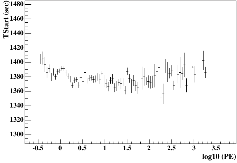
Figure 4.9: Calibrated TStart as a function of PEs. The statistics are poor at very high and very low PE values.
