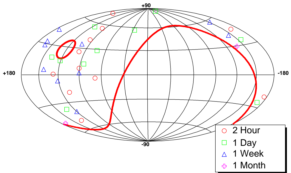
Figure 7.11: Locations in galactic coordinates of the most significant alerts between MJD 52332 and 53111. The boundaries of the search at \text{DEC}=0^\circ and \text{DEC}=80^\circ are marked by the red lines.
