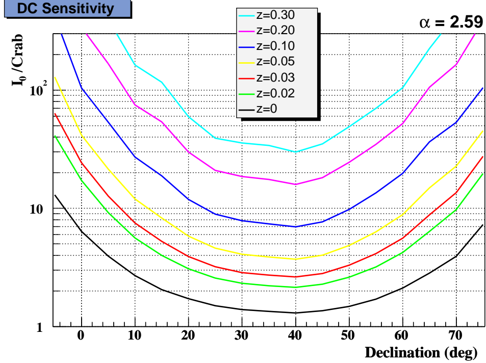
Figure 6.9: Photon flux amplitude, I_0 , in Crab units required to get a 5\sigma/\sqrt{y\tau} excess for a source at a given redshift as a function of declination. 1 year = 332 days of exposure. The assumed spectrum is dN/dE \propto E^{-2.59}e^{-\tau} with \tau calculated using IR1a.
