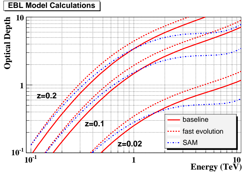
Figure 2.5: Optical depth of the universe to very high energy photons for several redshifts using three models of the EBL. Baseline and fast evolution from de Jager & Stecker (2002) and SAM for LCDM (Salpeter) from Primack et al. (1999). When the optical depth is 1, the photon survival probability is 1/e .
