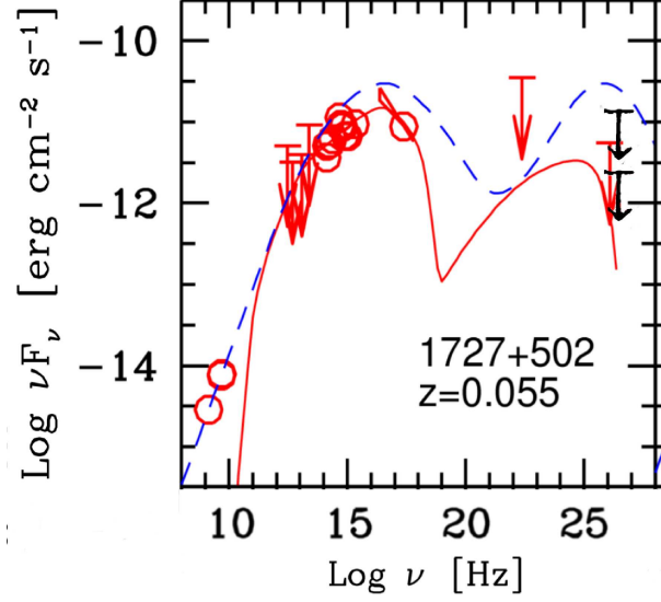
Figure 8.4: SED data and predicted SSC (solid) and Fossati (dashed) fits for I Zw 187 from Costamante & Ghisellini (2002). Upper limits in red for the second component are from Beppo Sax or IACT observations. The Milagro flux upper limits for an unabsorbed (lower) and absorbed (higher) spectrum are in black.
