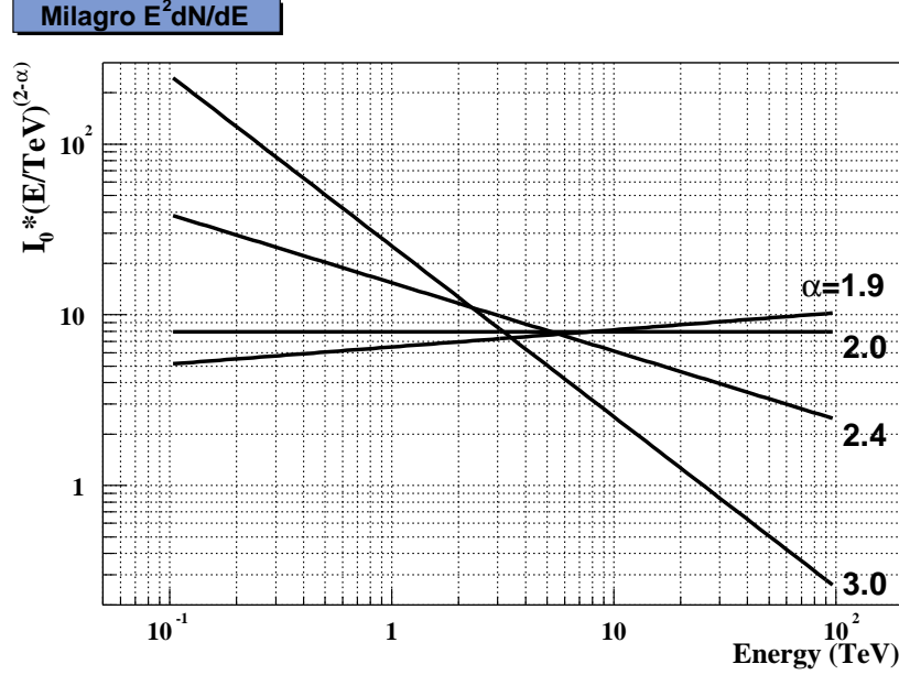
Figure 6.5: E^2 dN/dE as a function of energy, where dN/dE = I_0(E/TeV)^{-\alpha} . I_0 is calculated from Monte Carlo simulations using the same Milagro event rate for each line and assuming different spectral indexes. The region where the lines intersect indicates the energy at which the energy flux is least dependent on the assumed spectrum. The center of this region is 4.3 \pm 1.4 TeV.
