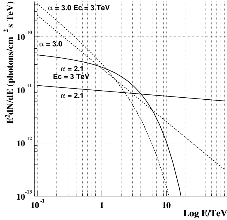
Figure 6.6: Differential flux dependence on the assumed energy spectrum. The plot shows E^2 dN/dE , where dN/dE = I_0(E/\text{TeV})^{-\alpha} e^{-E/E_c} . The exponential factor is dropped in the case of no cut-off energy. For each curve the event rate in the detector is chosen to be the same and the differential energy flux is calculated for different values of \alpha and the cut-off energy, E_c . The resulting values of I_0 for each combination are given in Table 6.2.
