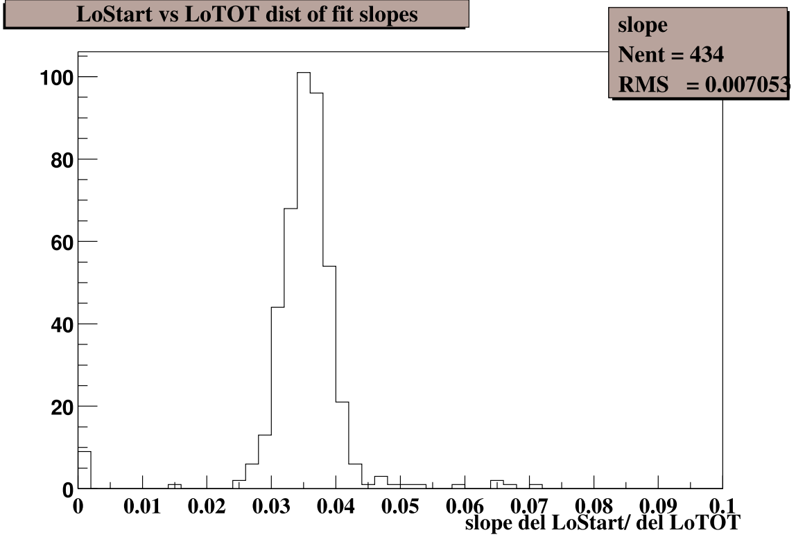
Figure 4.6: The results of fitting a line to slewing curves above 300 Lo TOT. The slope of the Lo TStart, Lo TOT data is shown for all AS PMTs with data. The distribution sets the range for a_1 and demonstrates the global similarities of the PMTs.
