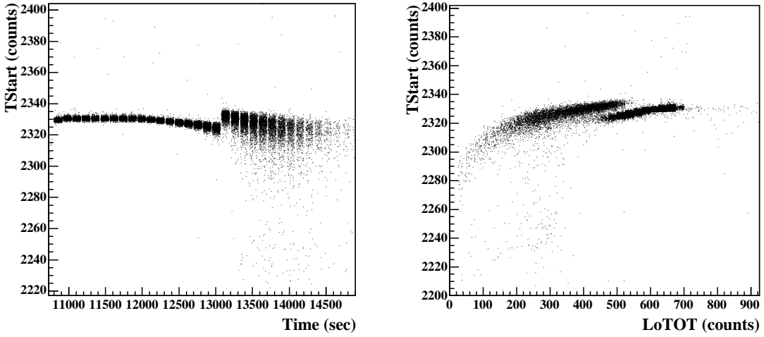
Figure 4.11: Example of a shift in time delay from the delay generator. The abrupt shift in TStart in the time plot (left) should not occur and causes a discontinuity in the slewing curve (right).
