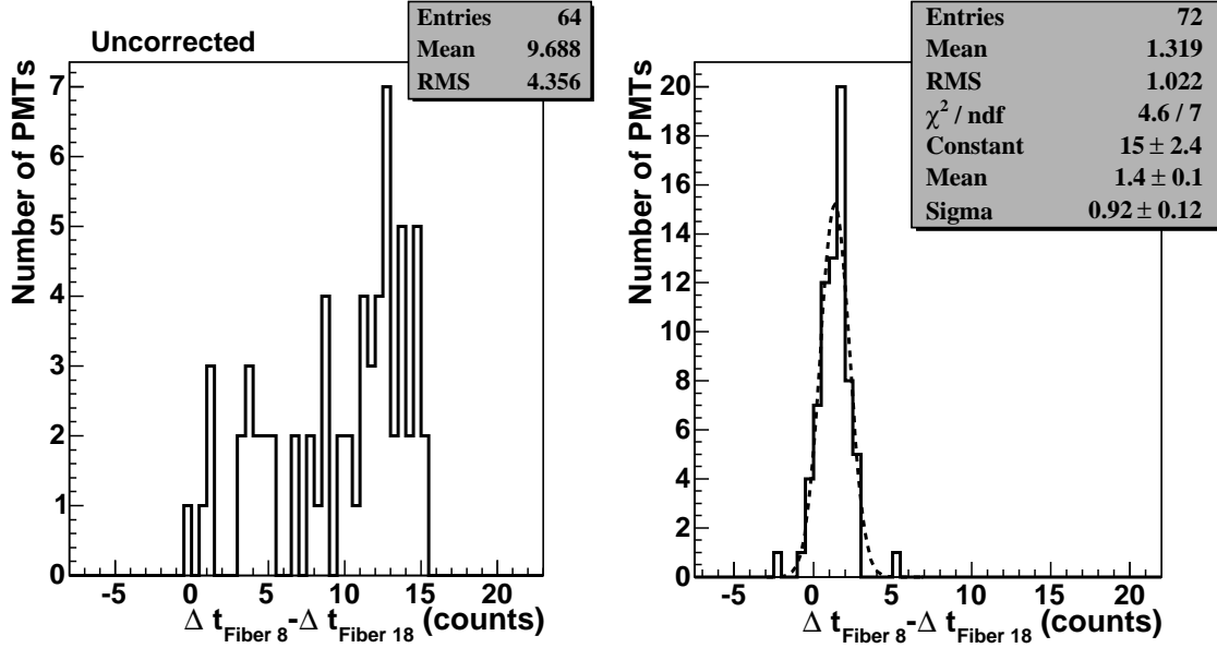
Figure 4.12: Distribution of \Delta t_{\text{Fiber}} differences for laser balls 8 and 18 before and after correcting the position of laser ball 18 in calibration data taken in November, 2001. The corrected distribution lists the parameters for a Gaussian fit.
