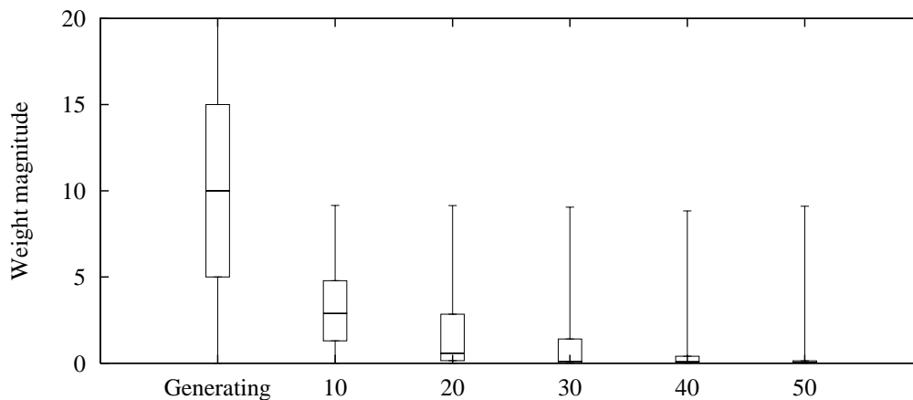
Figure 18. Box-whiskers plots showing the weight magnitude distribution for the generating network (10 hidden nodes, on the left) and the trained networks with 10 to 50 hidden nodes. Averaged over 10 trials in each case.
