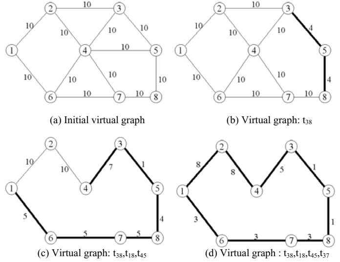
Figure 3. Virtual Graph after t_{48}
