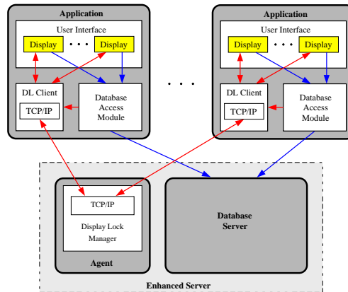
Figure 5. Implementation Architecture.
