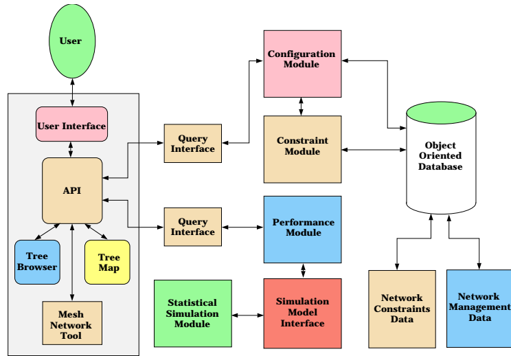
Figure 1. Architecture of the Integrated Network Management System.
