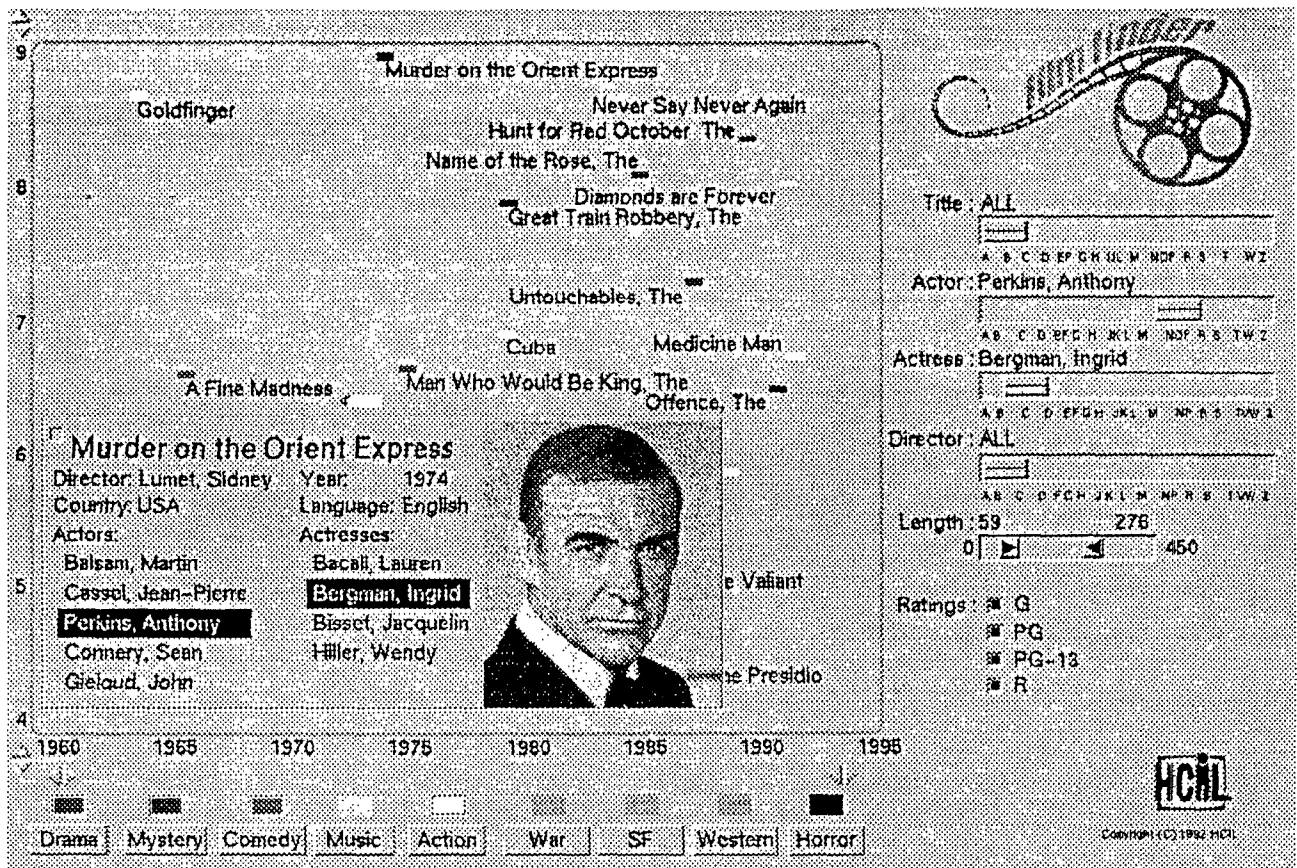
Ahlberg & Shneiderman, Color plate 3. Anthony Perkins and Ingrid Bergman has been selected in the information card - which is reflected in the Alphasliders.
