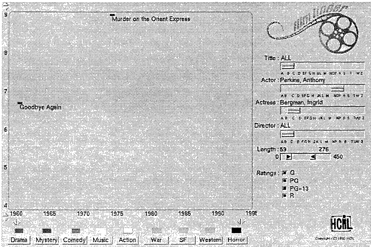
Ahlberg & Shneiderman, Color Plate 4. When the information card is closed the query result is updated to only include the movies starring both Anthony Perkins and Ingrid Bergman
