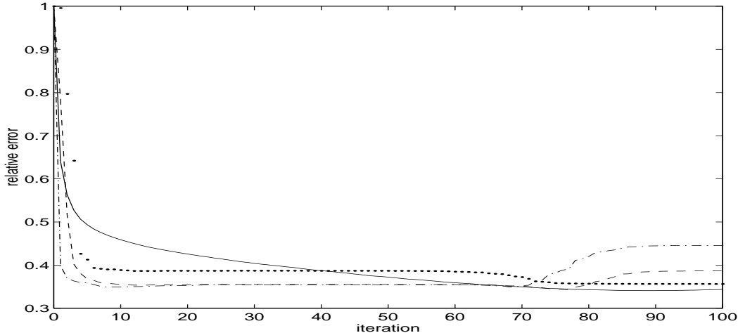
FIG. 4. Relative error in computed solutions for Example 1. Solid line shows convergence when m^* = 0 ; dashed line shows convergence for our preconditioner with m^* = 711 using the d -selection method; dotted line shows convergence when m^* = 583 using the Fourier coefficient selection method; dash-dotted line shows the convergence behavior for the preconditioning scheme in [13] with the cutoff at 725 eigenvalues.
