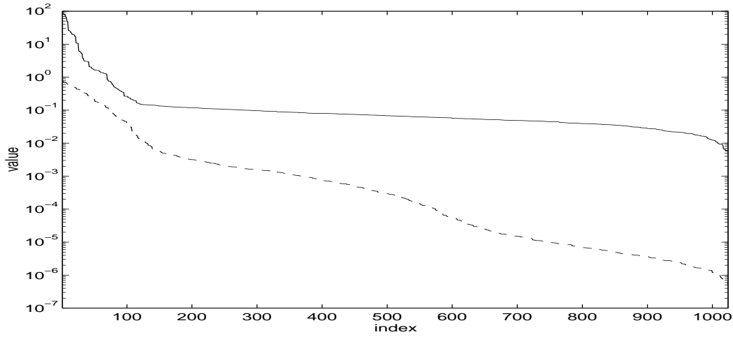
FIG. 7. Solid line shows 2-D Fourier coefficients of the noisy data sorted in order of decreasing magnitude. Dashed line shows diagonal entries obtained during factorization, sorted in order of decreasing magnitude, Example 2.
