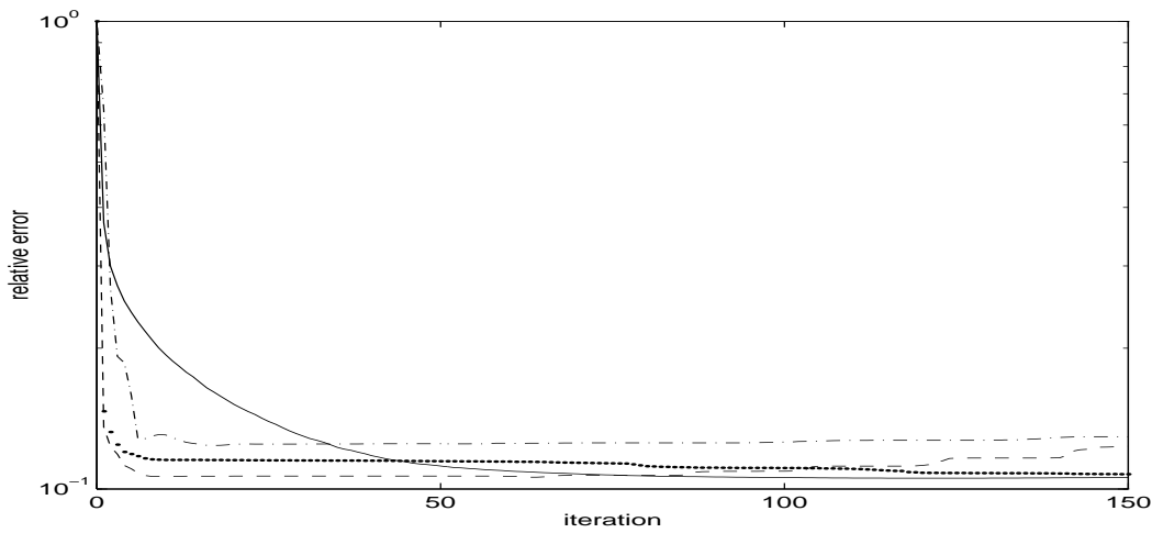
FIG. 11. Relative error in computed solutions for Example 3. Solid line shows convergence when m^* = 0 ; dashed line shows convergence for our preconditioner with m^* = 576 using the d -selection method; dotted line shows convergence when m^* = 435 using the Fourier coefficient selection method; dash-dotted line shows the convergence behavior for the preconditioning scheme in [13] with the cutoff at 574 eigenvalues.
