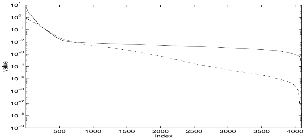
FIG. 3. Solid line shows 2-D Fourier coefficients of the noisy data sorted in order of decreasing magnitude. Dashed line shows diagonal entries obtained during factorization, sorted in order of decreasing magnitude, Example 1.
