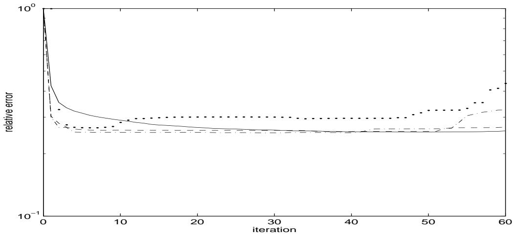
FIG. 8. Relative error in computed solutions for Example 2. Solid line shows convergence when m^* = 0 ; dashed line shows convergence for our preconditioner with m^* = 122 using the d -selection method; dotted line shows convergence when m^* = 109 using the Fourier coefficient selection method; dash-dotted line shows the convergence behavior for the preconditioning scheme in [13] with the cutoff at 116 eigenvalues.
