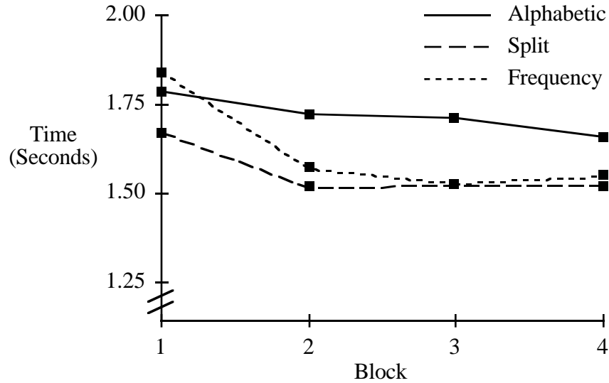
Figure 5: Average selection time vs. Block for three menu organizations for Distribution Two.
