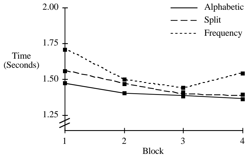
Figure 6: Average selection time vs. Block for three menu organizations for Distribution Three.
