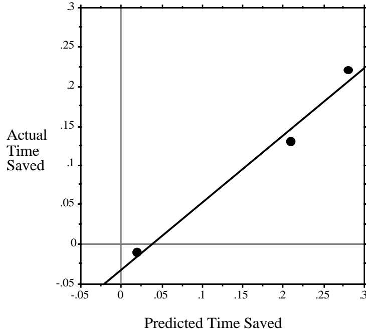
Figure 8: Predicted vs. Actual time saved (in seconds) for three distributions.
