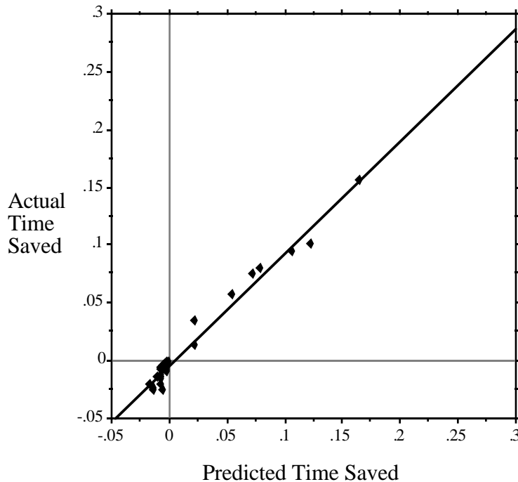
Figure 7: Predicted vs. Actual time saved (in seconds) for individual items.
