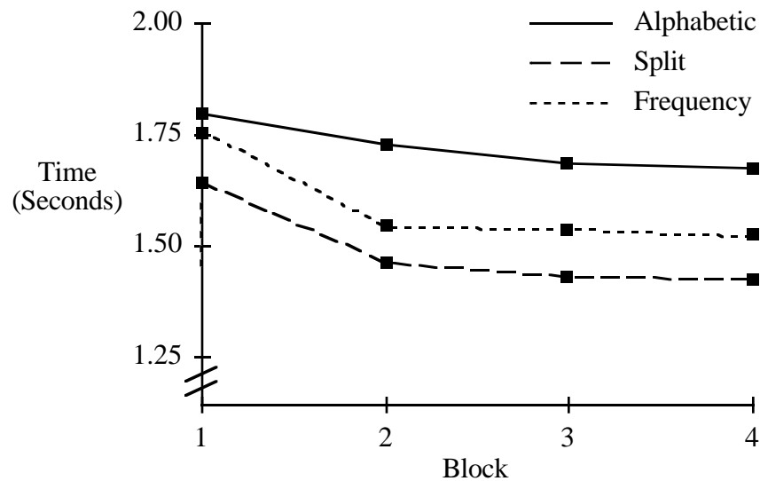
Figure 4: Average selection time vs. Block for three menu organizations for Distribution One.
