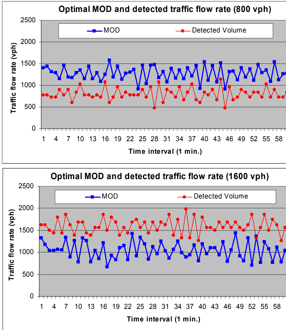
Figure 4.4.2 An Example of time-varying optimal control threshold (MOD)
