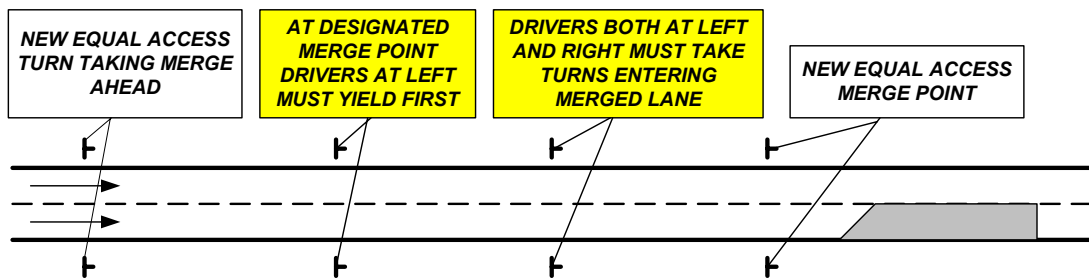
Figure 2.2.9 Configuration of equal excess merge
