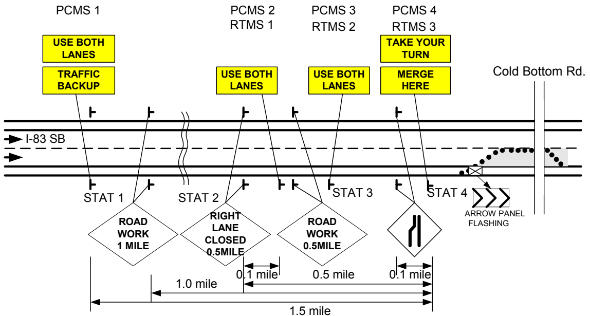
Figure 3.2.1 A Graphical illustration of the DLM and work zone
