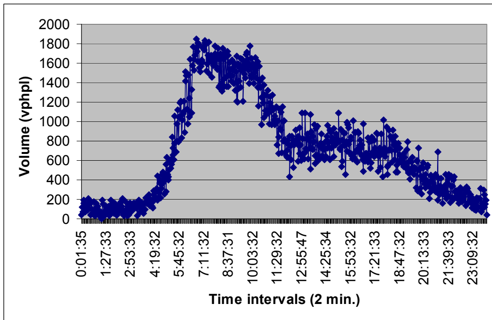
Figure 3.2.3 Traffic flow patterns under work-zone operations
