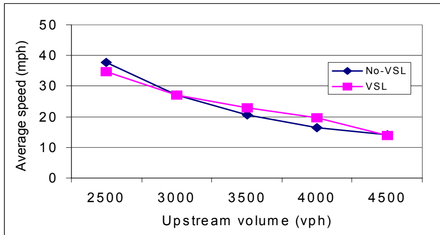
Figure 5.5.8 Average dpeed over subsegments for Type 2-1
