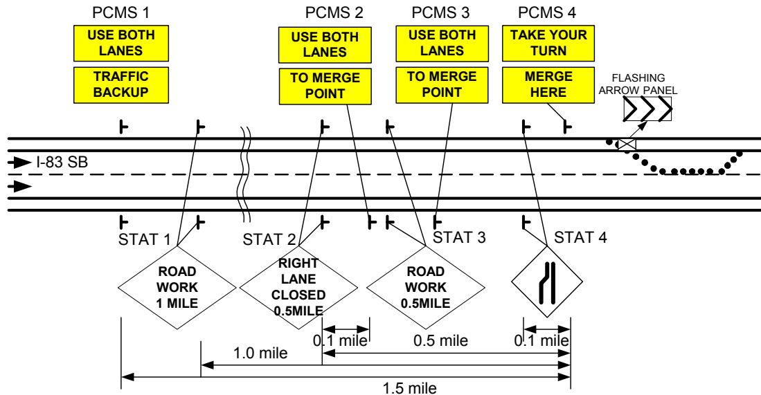
Figure 2.2.6 Configuration of the DLM system (MSHA: Maryland State Highway Admin.)
