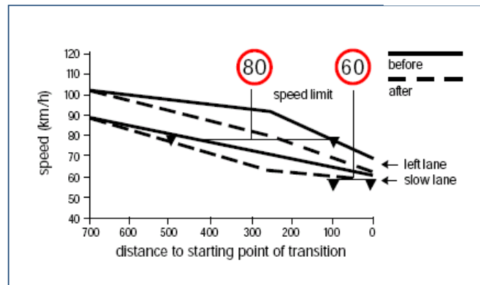
Figure 2.3.8 An Effect of narrow lane on reduced speed
