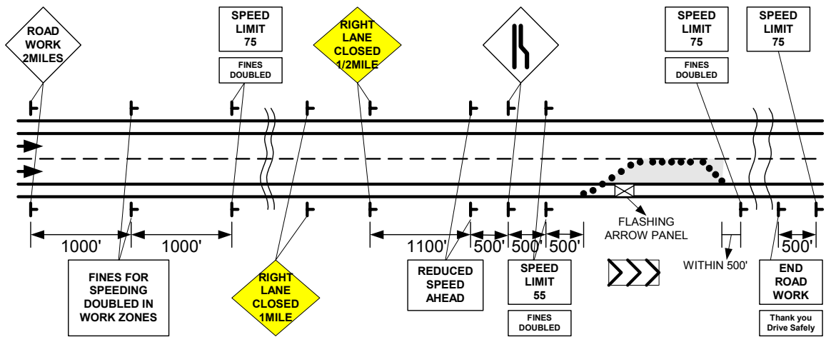
Figure 2.2.1 Configuration of the NDOR merge
