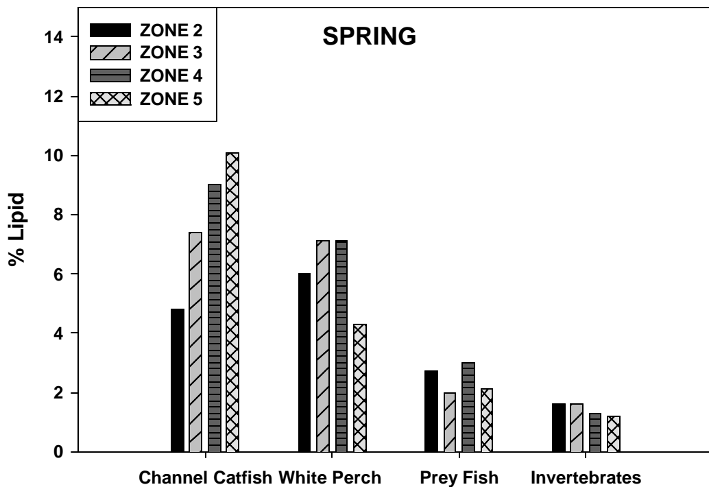
Figure 3.3. Percent lipid in biota collected from the Delaware River estuary in Fall 2001 and Spring 2002.
