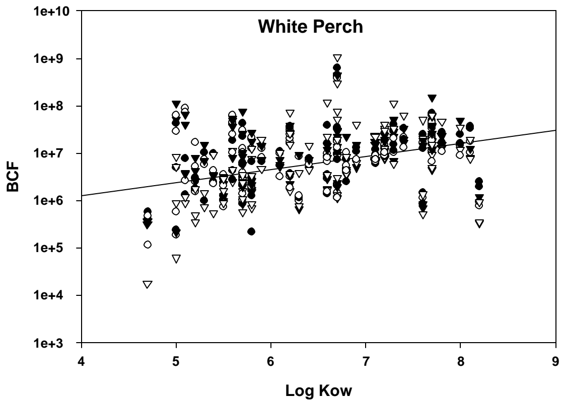
Figure 4.2. Bioconcentration factors (BCF) vs. log K_{ow} for individual PCB congeners in white perch collected from the Delaware River estuary, USA in Fall 2001 and Spring 2002. Regression analysis of BCF values vs. log K_{ow} values gave a linear regression of \log BCF = 0.25 \cdot \log K_{ow} + 5.24 ( R = 0.35 , P < 0.0001 ). ●=Zone 2, ○=Zone 3, ▼=Zone 4, ▽=Zone 5.
