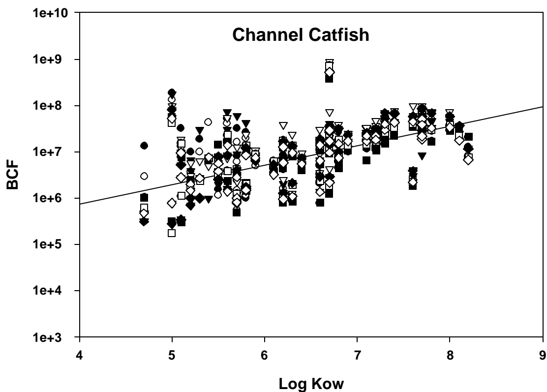
Figure 4.1. Bioconcentration factors (BCF) vs. log K_{ow} for individual PCB congeners in channel catfish collected from the Delaware River estuary, USA in Fall 2001 and Spring 2002. Regression analysis of BCF values vs. log K_{ow} values gave a linear regression of \log BCF = 0.34 \cdot \log K_{ow} + 4.81 ( R = 0.49 , P < 0.0001 ). ●=Zone 2, ○=Zone 3, ▼=Zone 4, ▽=Zone 5.
