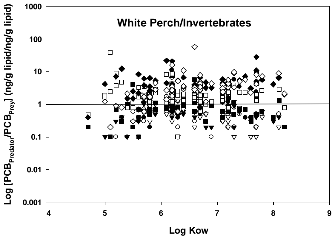
Figure 4.12. Lipid normalized predator/prey ratios vs. log K_{ow} for individual PCB congeners for white perch/invertebrates collected from the Delaware River estuary, USA in Fall 2001 and Spring 2002. The line represents a 1:1 ratio, indicating no bioaccumulation of PCBs from prey to predator. ●=Fall Zone 2, ○= Fall Zone 3, ▼= Fall Zone 4, ▽= Fall Zone 5, ■=Spring Zone 2, □=Spring Zone 3, ◆=Spring Zone 4, ◇=Spring Zone 5.
