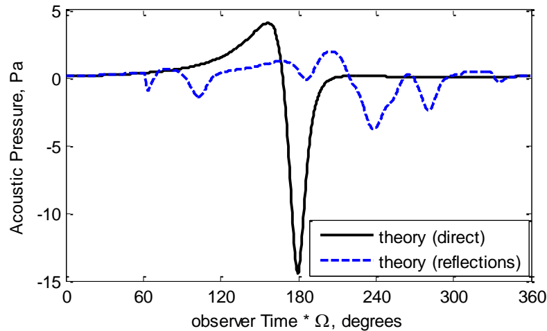
Figure 1.8: One-revolution time history of rotor harmonic noise
