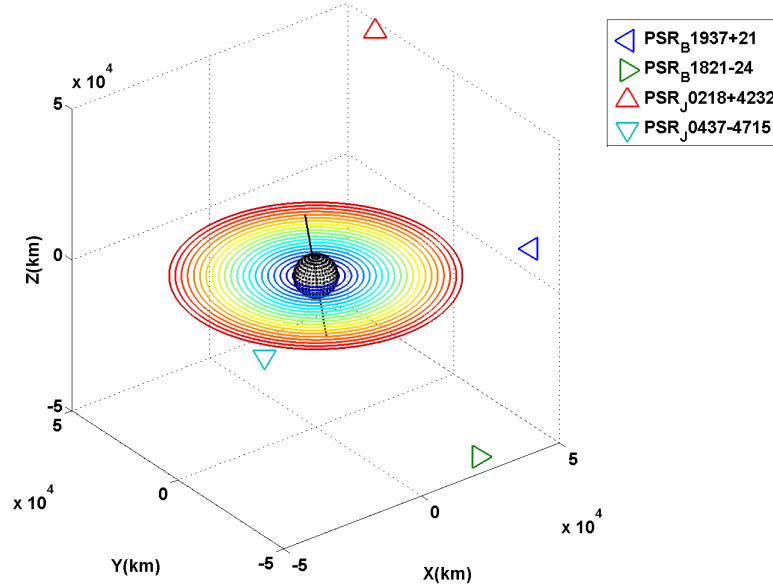
Figure 6.12: SMA Orbit Trade Space. Orbit trade value increases from blue (6678 km) to red (42158 km) for each trajectory.
