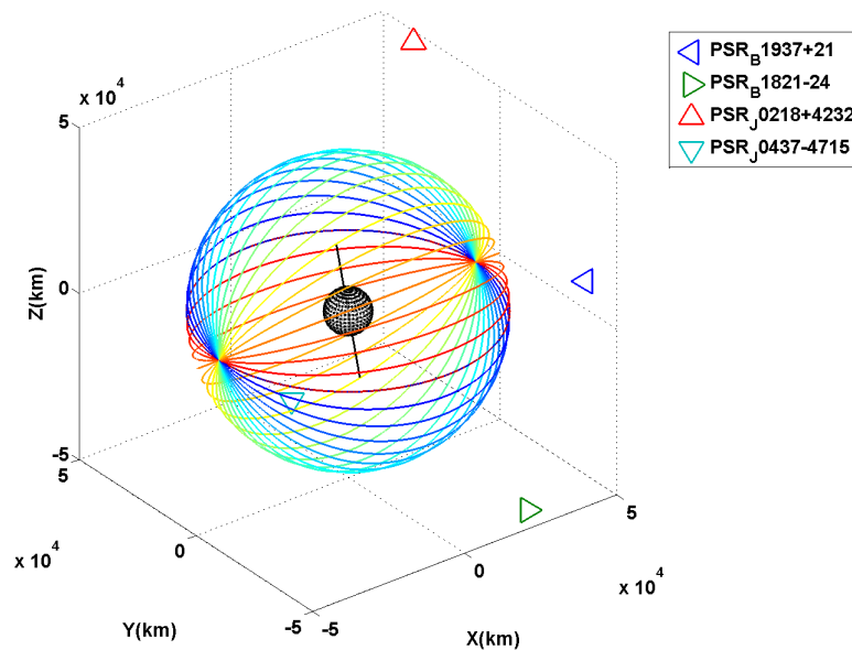
Figure 6.21: INC Orbit Trade Space. Orbit trade value increases from blue ( 0^\circ ) to red ( 180^\circ ) for each trajectory.
