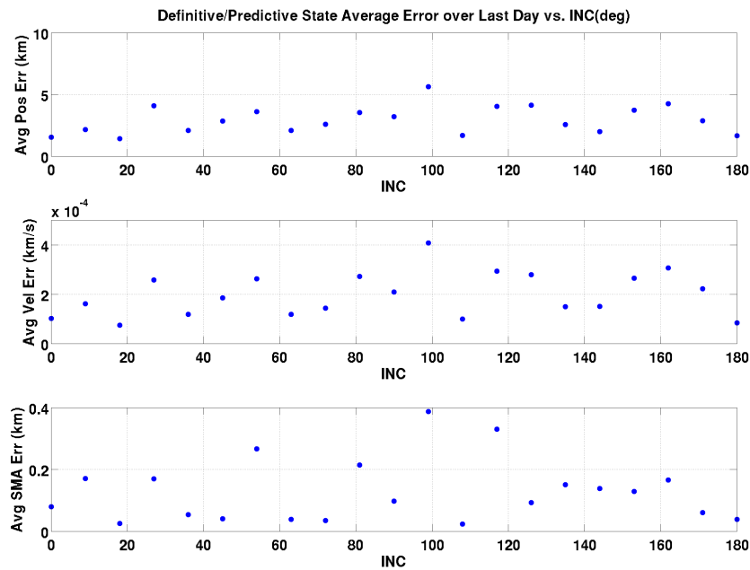
Figure 6.22: Average State Error vs. INC. 42158 km SMA Circular Orbit.
