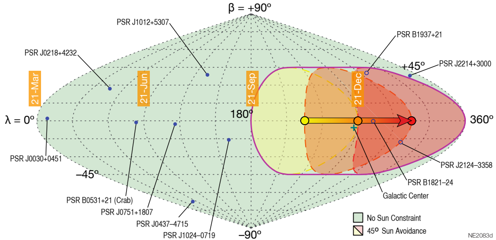
Figure 3.9: A diagram of the distribution of possible MSPs in the galactic ecliptic frame [39].
