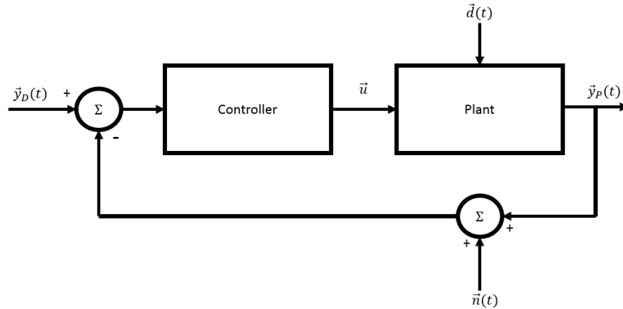
Figure 2.13: Single Loop Feedback Control Loop
