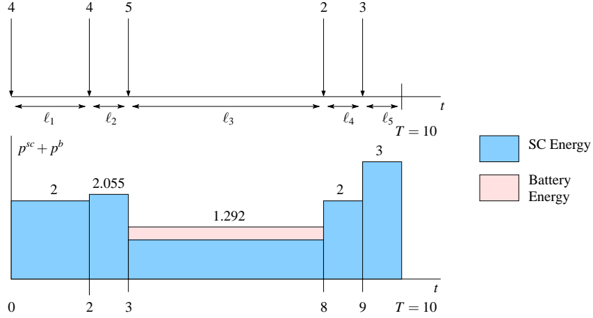
Figure 5.1: Optimal transmit powers for hybrid storage with E = [4, 4, 5, 2, 3] mJ at times t = [2, 3, 8, 9] sec, \eta = 0.75 , E_{max} = 5 mJ and T = 10 sec.
