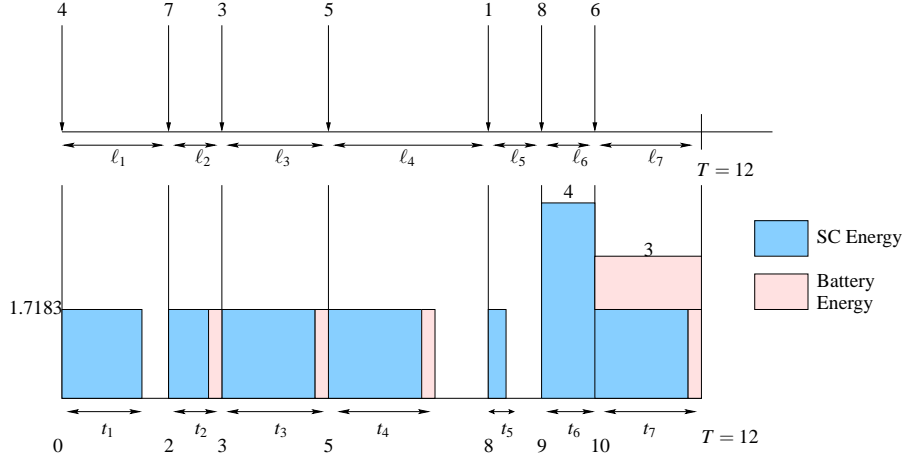
Figure 5.2: Optimal transmit powers for E = [4, 7, 3, 5, 1, 8, 6] mJ at times t = [2, 3, 5, 8, 9, 10] sec, \eta = 0.75 , E_{max} = 5 mJ, \epsilon = 1 and T = 12 sec.
