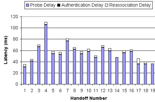
Figure 7: Handoff Latencies - Lucent STA with Cisco AP
