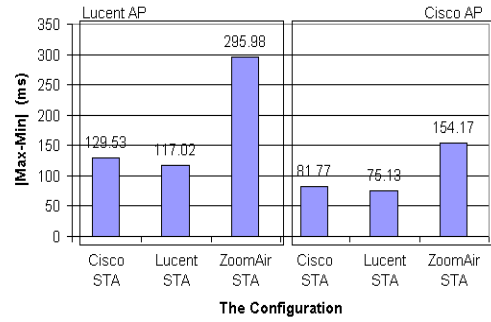
Figure 13: The Max-Min for various handoff latencies.
