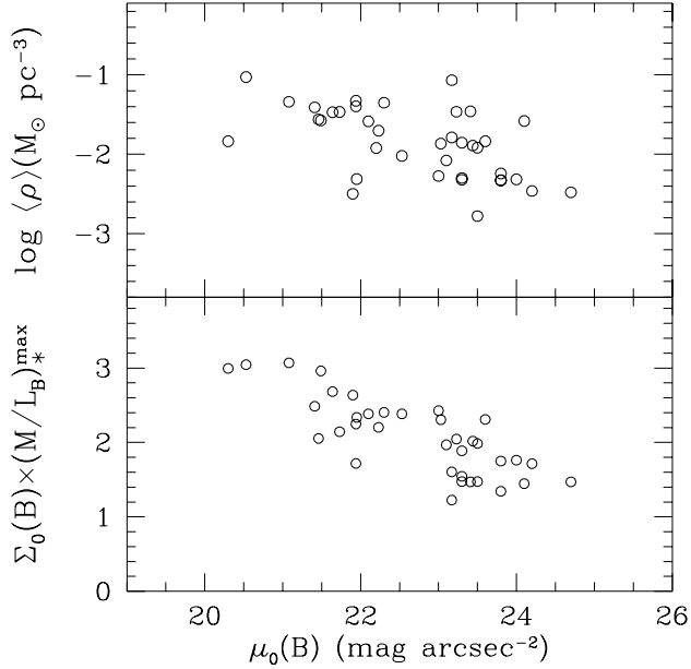
Figure 12. Top panel: Average volume density of LSB galaxies as measured within 5 disk scale lengths. Bottom panel: Central mass surface density implied by the maximum disk fits. Both quantities depend on surface brightness.
