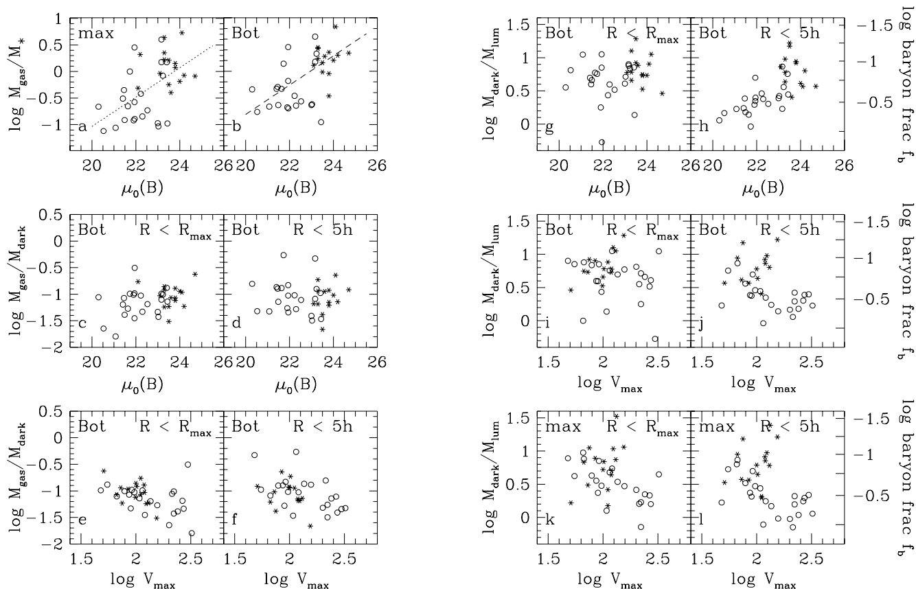
Figure 11. Ratios of the various mass components. All stellar and dark masses are computed as indicated in the panels, where ‘max’ denotes maximum disk and ‘Bot’ Botttema disk. The outermost radius R_{\max} is defined as the the radius of the last measured point of the rotation curve. h is the disk scale length. Shown are: the ratio of stellar masses and gas masses for maximum disk (a), where the dotted line is a least-squares fit to the data; the ratio of stellar masses and gas masses for Botttema disk (b); the ratio of gas mass and dark mass as a function of surface brightness \mu_0 , measured within R_{\max} (c) and within 5h (d); the ratio of gas mass and dark mass as a function of maximum rotation velocity V_{\max} , measured within R_{\max} (e) and within 5h (f); the ratio of dark mass and luminous mass (and baryon fraction) as a function of \mu_0 , measured within R_{\max} (g) and within 5h (h); the ratio of dark mass and luminous mass for the Botttema disk as a function of V_{\max} , measured within R_{\max} (i) and within 5h (j); the ratio of dark mass and luminous mass for the maximum disk as a function of V_{\max} , measured within R_{\max} (k) and within 5h (l)
