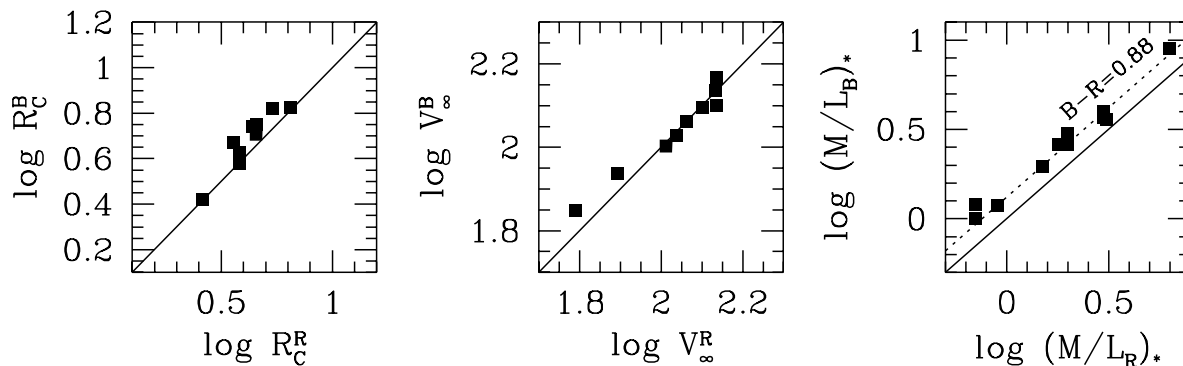
Figure 6. Comparison of the core radii R_C (left panel) and asymptotic velocities (middle panel) V_\infty of the halos, and the maximum disk mass-to-light ratio (M/L)_* of the stellar disk (right panel) resulting from separate B and R band decomposition of the rotation curves of the subset of LSB galaxies for which both R and B band photometry were available. The B and R band decompositions are consistent with each other. The full drawn lines are lines of equality. The dotted line in the right panel is the relation between (M/L_B)_* and (M/L_R)_* for B - R = 0.88 .
