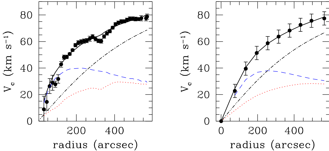
Figure 4. High and low resolution rotation curves of NGC 1560. The left panel shows the original high resolution observation from Broeils (1992). The curves measures 38 beams, and is well-resolved. The right panel shows the same data but smoothed to a resolution of only 3 beams. It is striking that the overall shape and amplitude of the curves have remained virtually unchanged. This is discussed more fully in Section 3.3. The dashed and dotted lines show the maximum disk decompositions for both cases. The dotted lines represent the rotation curve of the gas component, the dashed lines the rotation curve of the maximum stellar disk. The dash-dotted lines are the rotation curves of the halos as derived from this decomposition. There is almost no difference between the low- and high-resolution halo parameters. This is discussed more fully in Section 5.1. The fitting parameters are given in Table 6.
