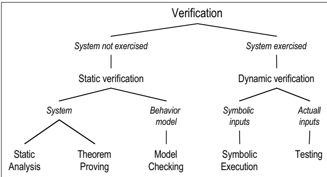
Figure 5.4: Verification approaches
