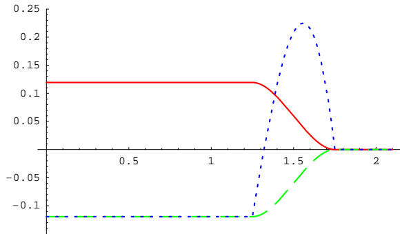
FIG. 1. The distribution of the matter defined by equations (2.3) and (2.5). The solid curve is the energy density \rho(r) , while the dashed curve is the radial stress P_r(r) in the same units. The dotted curve is P_\perp(r) , the transverse stress. Note that for r \leq 5/4 the stress energy tensor reduces to a false vacuum condition (cosmological ‘constant’) since P_r = P_\perp = -\rho .
