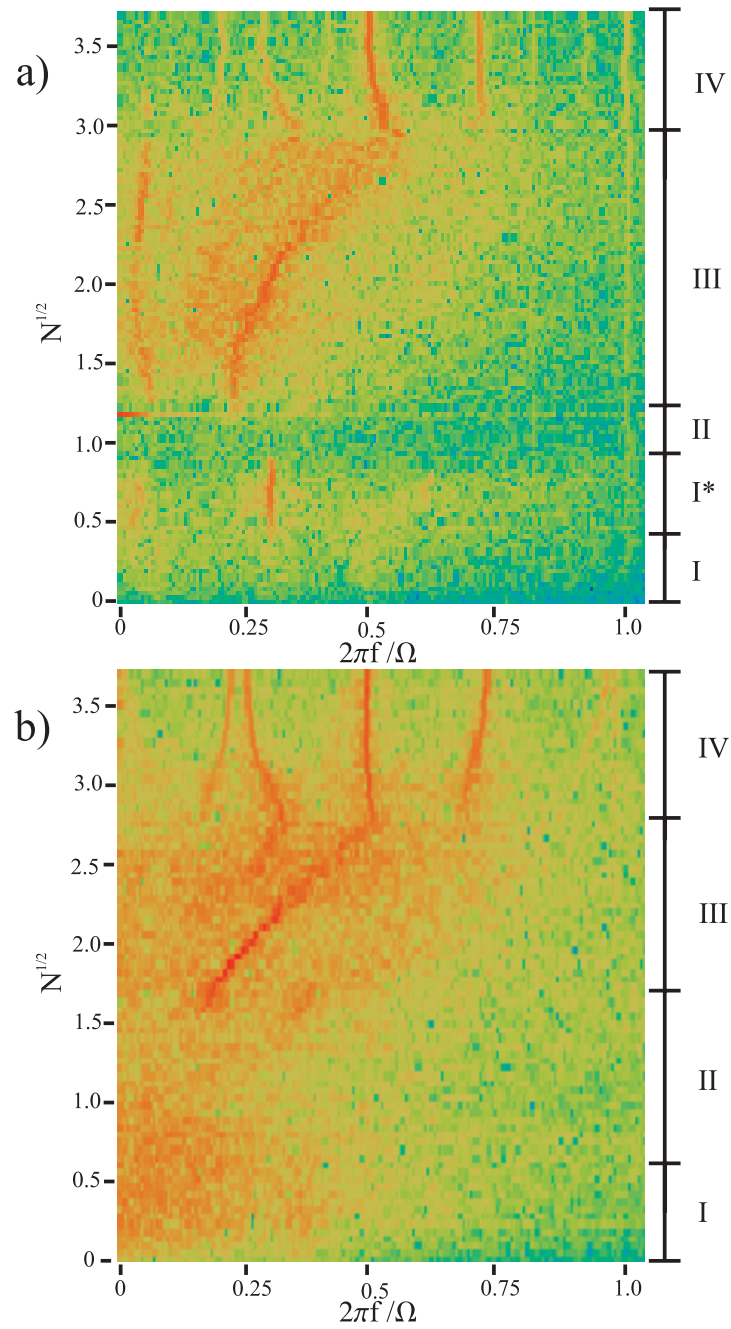
Figure 5.2: Induced field power spectra. Applied field increases up the page, where each horizontal line is a power spectrum of the induced field for smooth walls (a) and with baffles (b). Color indicates logarithmic intensity, from highest to lowest: red-yellow-green-blue. The impeller rotation rate is 10 Hz ( Re_m = 7.5 ).
