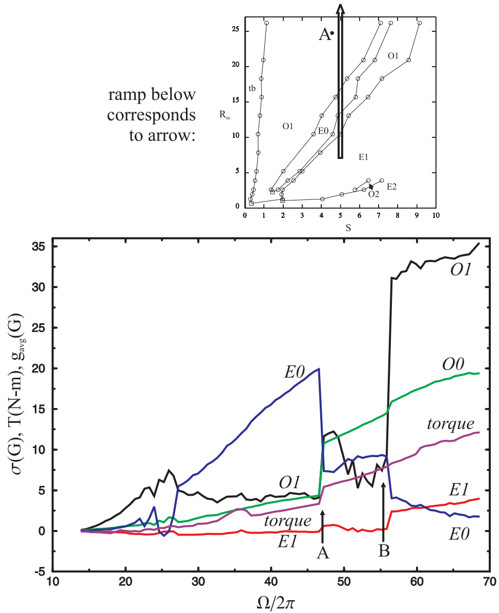
Figure 4.16: Torque, mode standard deviation (for m \neq 0 ), and mode average value (for m = 0 ) versus rotation rate for B_{ext} = 1000 \text{ G} . At the starting rotation rate (14 Hz), all values have been artificially set to zero. The field was turned on and then the motors. The field decreases approximately 50 G over the ramp due to coil heating.
