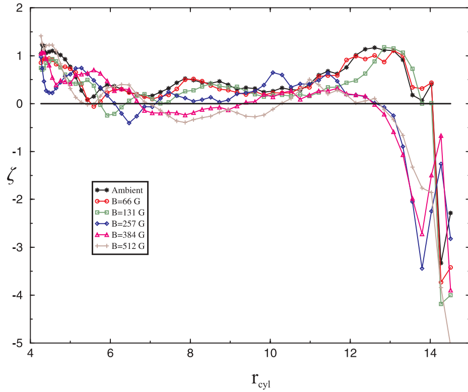
Figure 4.23: Profiles of the index \zeta \sim 2 + d \ln \Omega(s) / d \ln s for \Omega / 2\pi = 30 Hz, for five values of applied field. As the applied field increases, the \zeta profiles make more frequent excursions below \zeta = 0 , the threshold for centrifugal stability.
