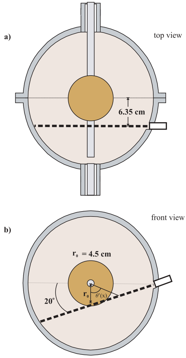
Figure 3.7: The location of the ultrasound measurements, which were along one chord. The angle \theta'(x) is used to calculate the cylindrical radial and azimuthal components.
