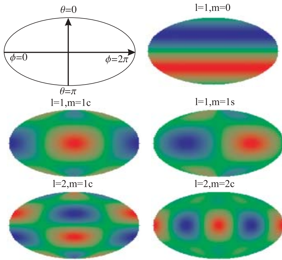
Figure 3.5: Cylindrical radial component of several coefficients on the surface of a sphere, in an equal area projection. Color represents intensity: red (positive), blue (negative), green (null).
