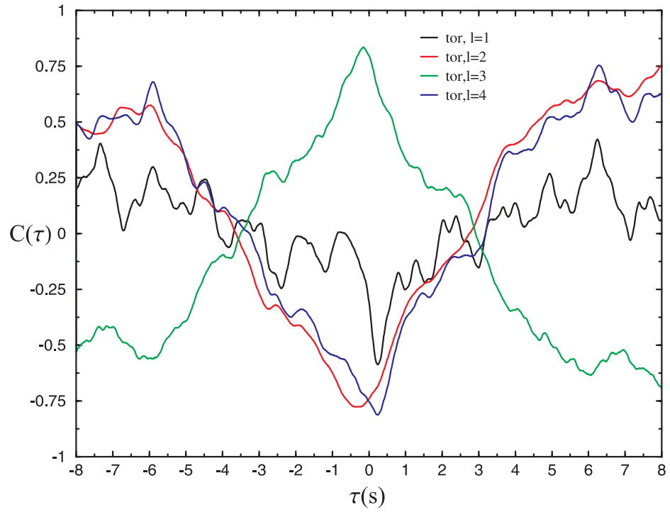
Figure 4.26: Cross-correlation function between torque and m = 0 coefficients, for \Omega/2\pi = 40 Hz. The l = 3 state is strongly correlated, while the l = 2, l = 4 states are strongly anti-correlated. No strong correlations exist between the torque and any other observed Gauss coefficients. Furthermore, at other parameter values the torque is only very weakly correlated ( C < 0.25 ) with all the Gauss coefficients.
