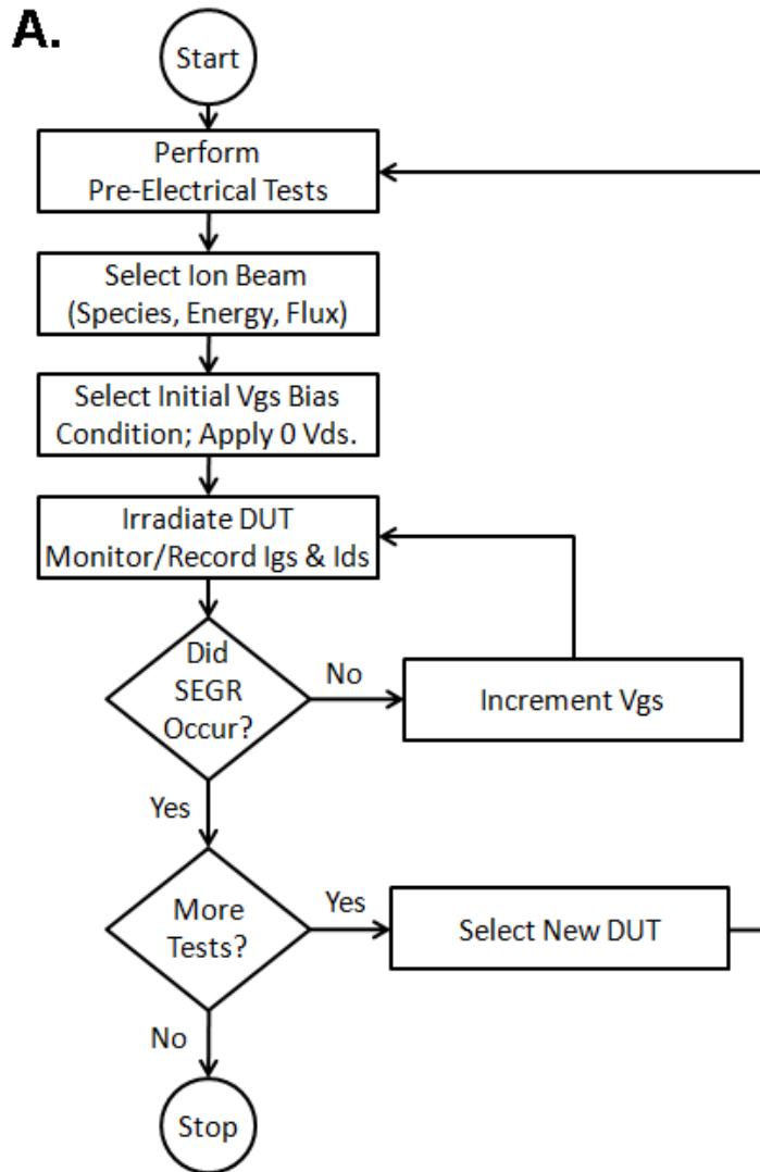
Figure 3.1. A: Flowchart depicting test procedure, after [47]. Note the absence of a post-irradiation gate stress test due to the high-magnitude Vgs bias conditions during irradiation. B: Test circuit diagram. C. TAMU operator control room with test equipment. D. Test board with DUT in line with beam.
