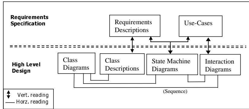
Figure 2 – Reading Techniques used in the experiment
