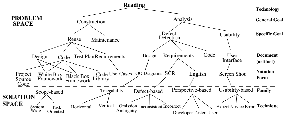
Figure 1 – Families of Reading Techniques
